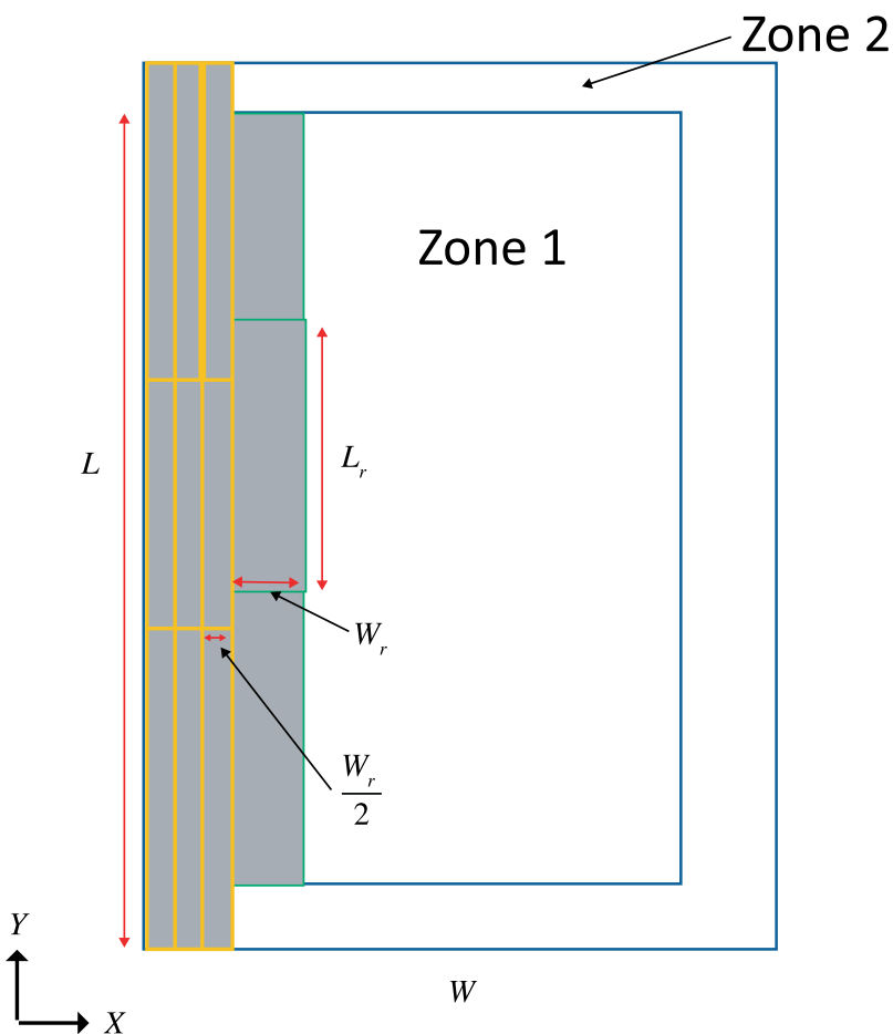
Figure 3. Roof zone layout with variables defined for use in the calculator.
